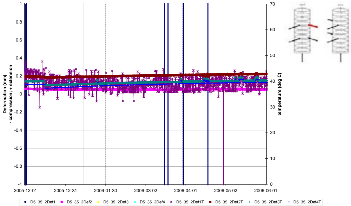
Deformation measurements Borehole D5:3.5(2)
