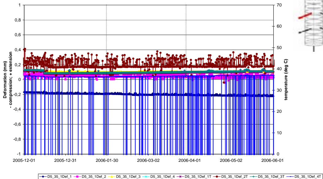
Deformation measurements Borehole D5:3.5(1)
