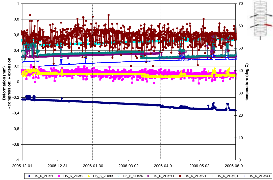
Deformation measurements Borehole D5:6(2)
