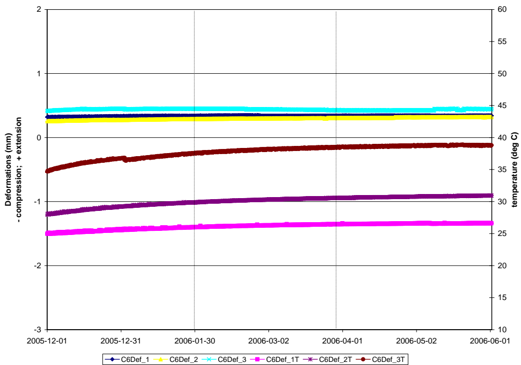
Vertical deformations adjacent to Deposition Hole 6 in borehole C6
