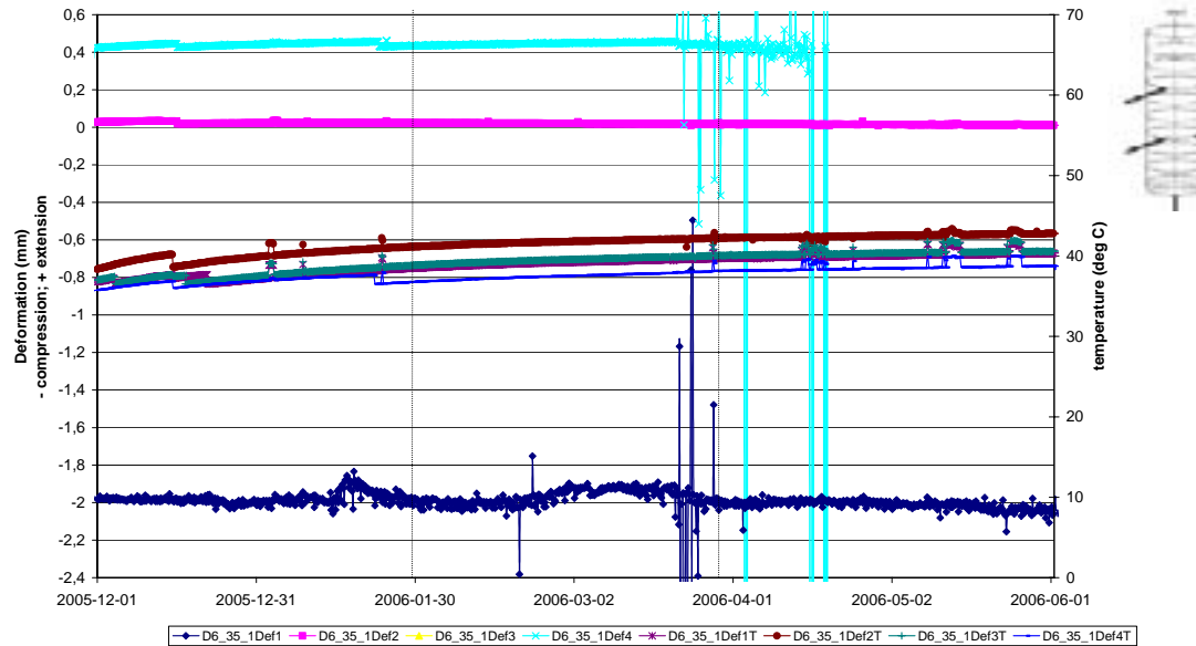
Deformation measurements Borehole D6:3.5(1)
