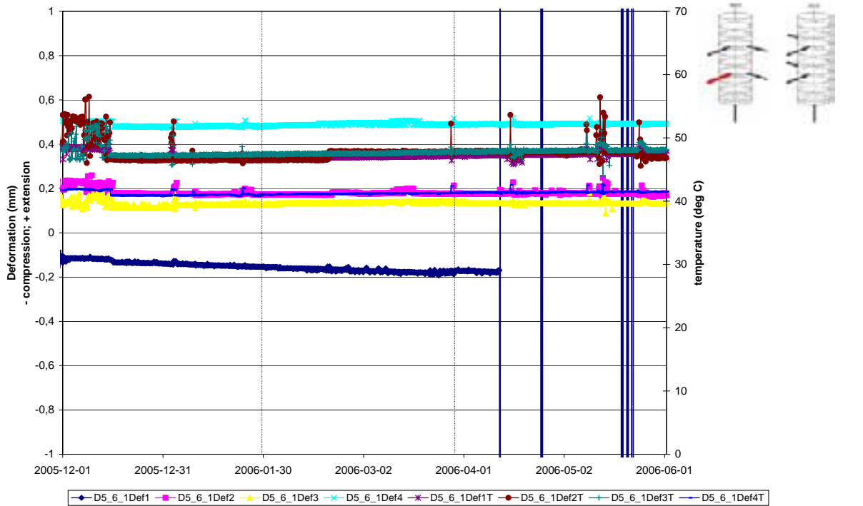
Deformation measurements Borehole D5:6(1)
