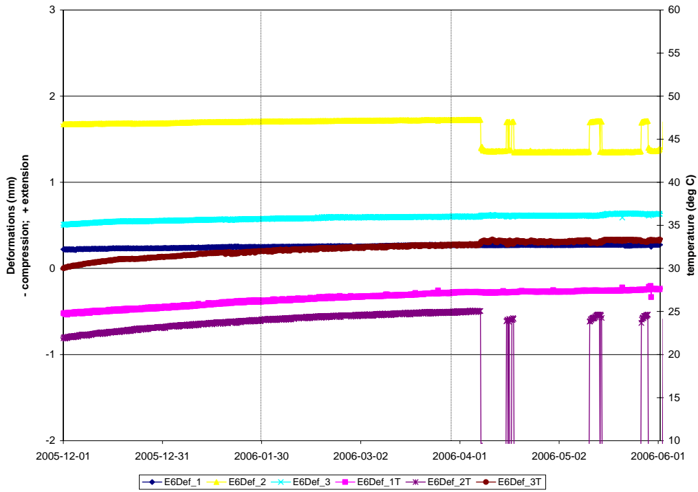
Vertical deformations adjacent to Deposition Hole 6 in borehole E6
