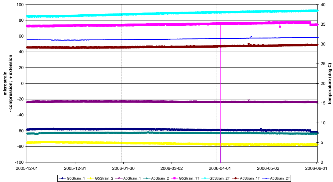
Vertical strain adjacent to Deposition Hole 5
