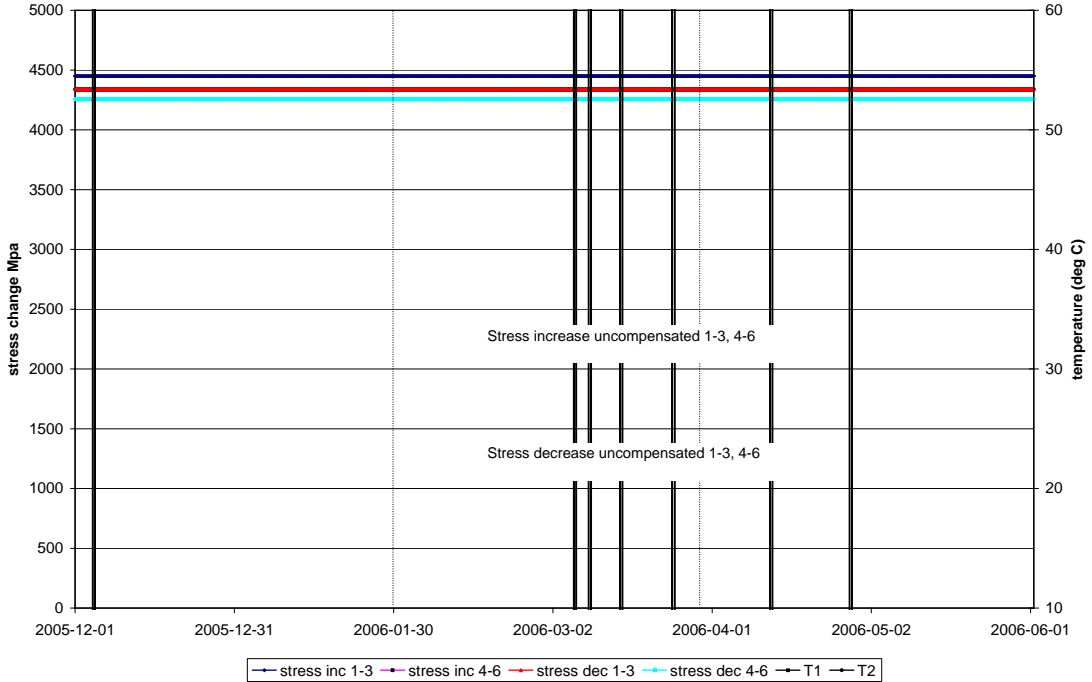
Biaxial stressmeter C6 Maximum stress increase and stress decrease in plane perpendicular to borehole axis
