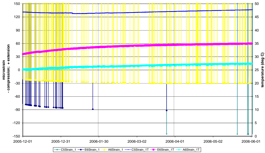
Vertical strain adjacent to Deposition Holes 5 and 6
